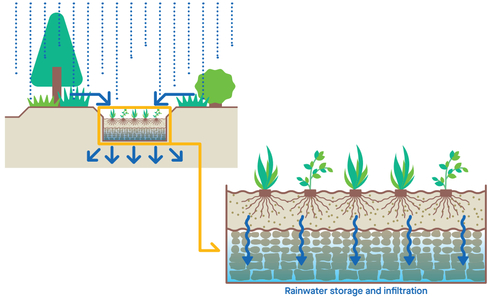
Mechanism of rain garden
