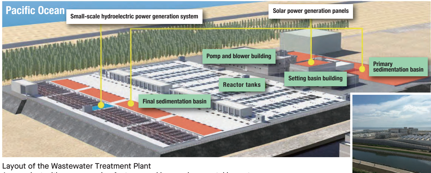
Minami-Gamo Wastewater Treatment Plant
